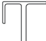
F Trim US44 47.5 X 45.5 mm (1.9 X 1.8 in)
