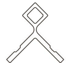
Outside Corner Trim UH51 75 x 77.5 mm (3.0 x 3.1 in)
