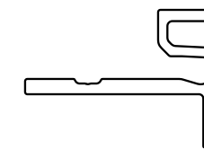
End Trim UH50 75 x 54 mm (3.0 x 2.1 in)
